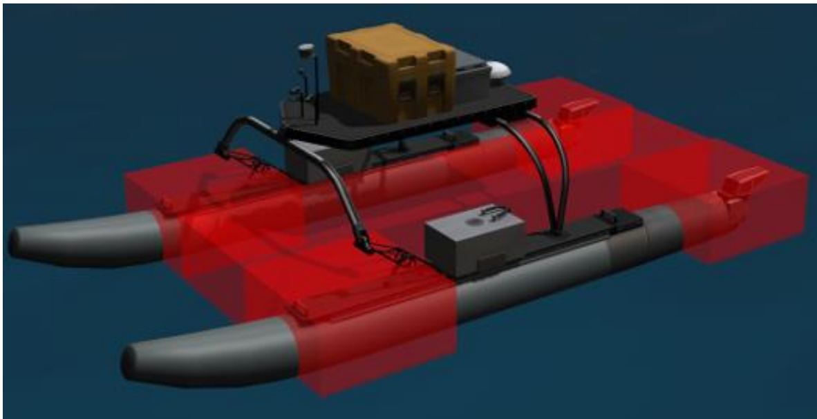
Figure 2: Allowed thruster regions in WAM-V
